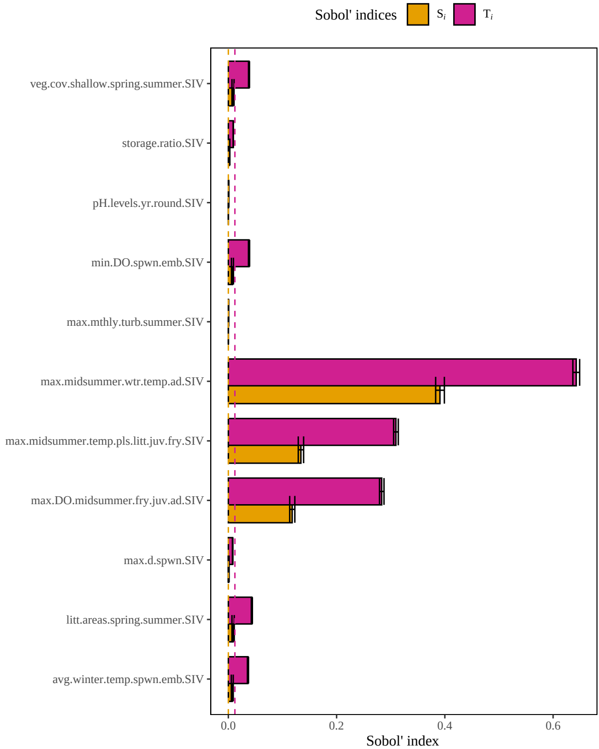
Figure 3. Results of a sensitivity analysis for the commoncarpLacNoSal model based on the original author-specified model outlined in Edwards and Twomey (1982). Dashed lines represent baseline numerical approximation error for S_i and T_i ( i.e. , dummy variables).
