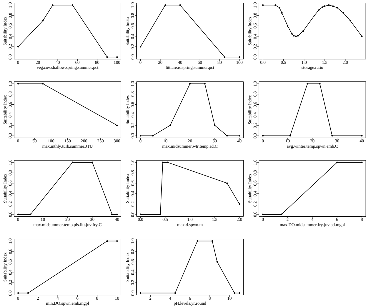
Figure 1. Suitability index graphs for variables included in the commoncarpLacNoSal model in ecorest.
